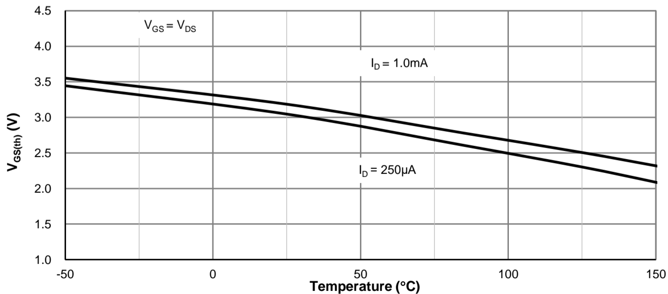
Figure 5: V_{GS(th)} vs. Junction Temperature
